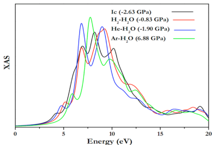
Figure 2. Calculated oxygen K-edge XAS on ice Ic phase, \text{H}_2\text{-H}_2\text{O} , \text{He-H}_2\text{O} , and \text{Ar-H}_2\text{O} .
